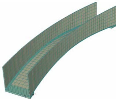
Fig. 2 Finite element mesh
