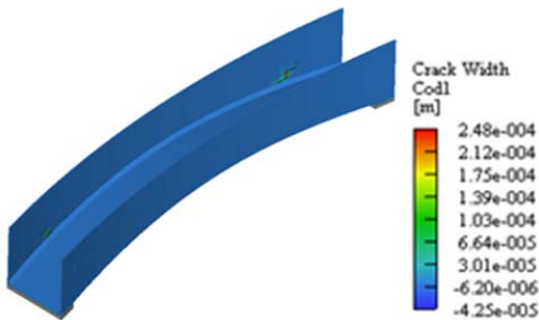
Fig. 7 Cracks for the structure before failure, the applied force of 4.2 kN/m 2 , the maximum crack width 0.248 mm
