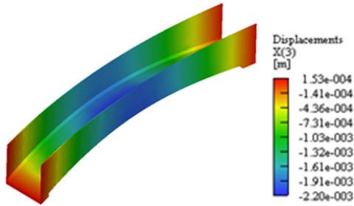
Fig. 6 Vertical deflection of the structure before failure, the applied force of 4.2 kN/m 2 , the maximum deflection value -2.2 mm
