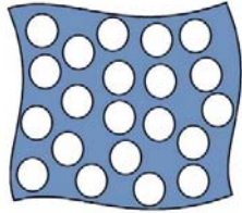
Fig. 2 Periodic boundary conditions
