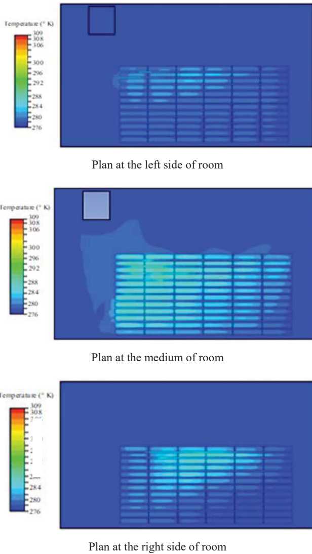
Fig. 4 Distribution of temperature after 25 hours of cooling for three positions in room
