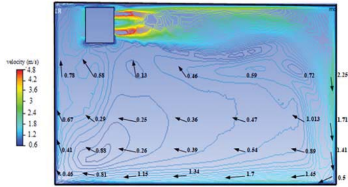
Fig. 2 Air flow
