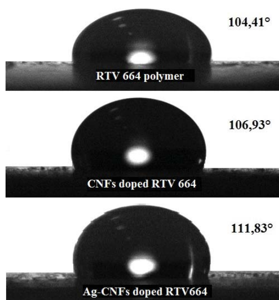
Fig. 7 Contact angles of polymer composite samples
