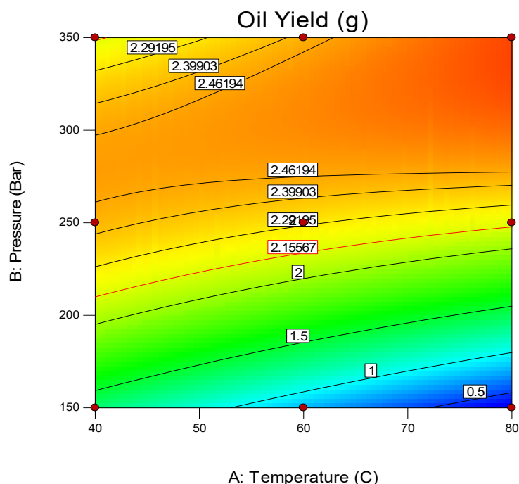
Fig. 3 Contour plot of the experimental data extraction soybean oil from modified supercritical carbon dioxide
