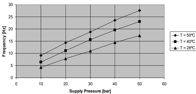
Fig. 6 System supply pressure at different temperatures
