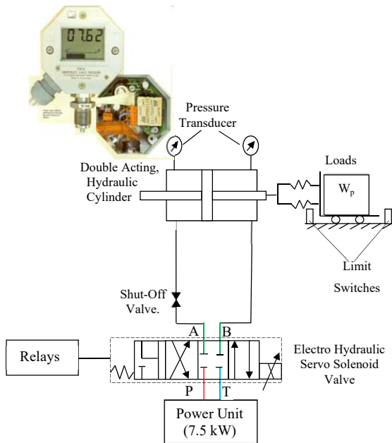
Fig. 3 Hydraulic circuit of fluid power control system (7.5 kW)
