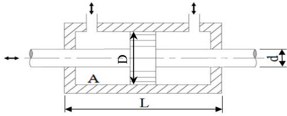
Fig. 1 Schematic drawing of double acting, double rod hydraulic cylinder. ID = 80 mm, d = 45 mm, L = 190 mm, p_{max.} = 210 bar, A = 3436.116965 mm 2
