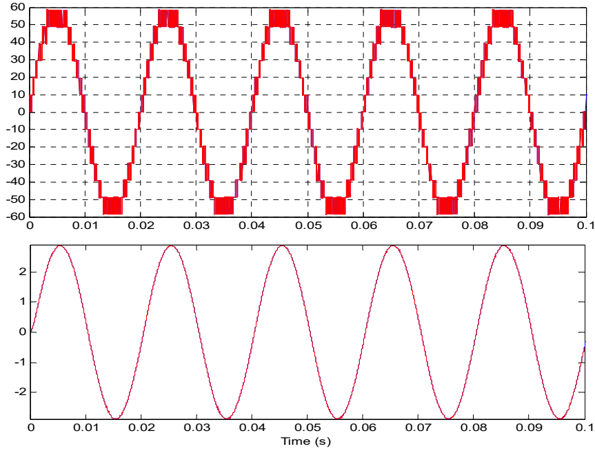
Fig. 8 Output voltage and current waveforms for R=20\ \Omega & L=10\ \text{mH}
