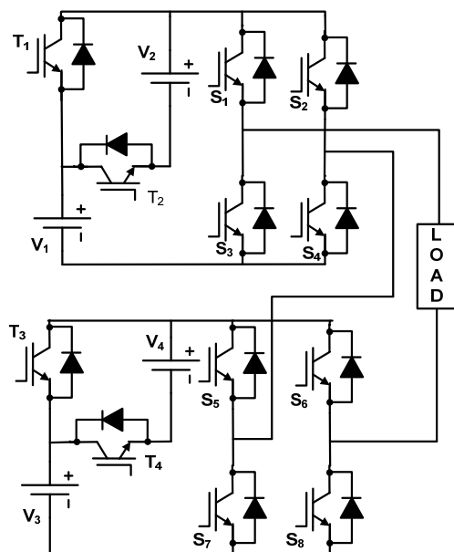
Fig. 1 Proposed thirteen-level inverter topology
