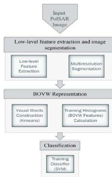
Fig. 2 Flowchart of the proposed algorithm
