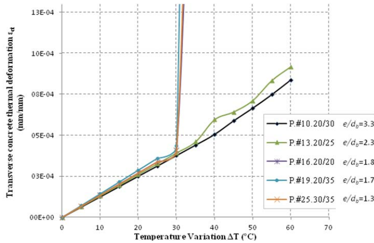
Fig. 4 Transverse concrete thermal deformation at external surface of concrete cover of concrete beam reinforced with two FRP bars having different ratio e/d_b
