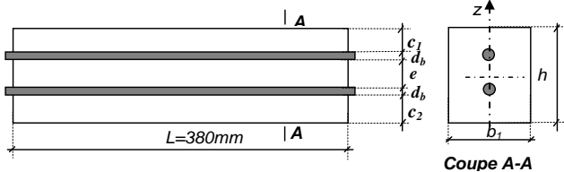
Fig. 1 Concrete beam reinforced with 2 GFRP bars modeled
