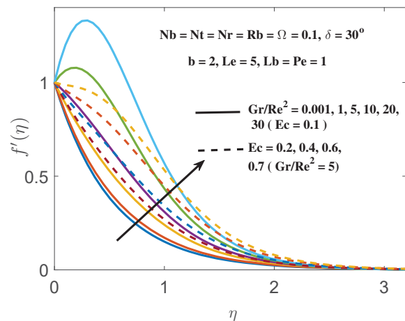
Fig. 3 Impact of \frac{Gr}{Re^2} and Ec on f'(\eta)
