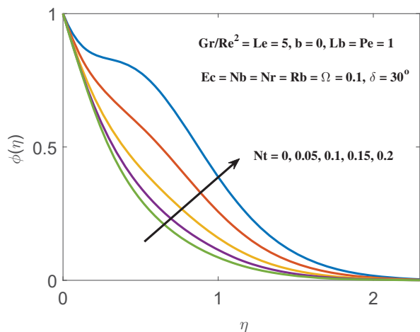
Fig. 12 Impact of Nt on \phi(\eta)
