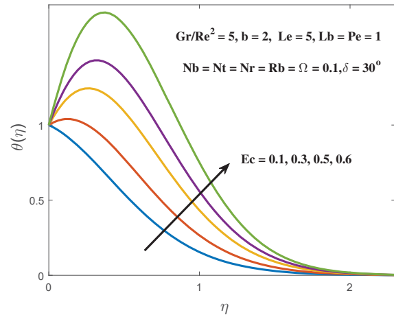
Fig. 7 Impact of Ec on \theta(\eta)
