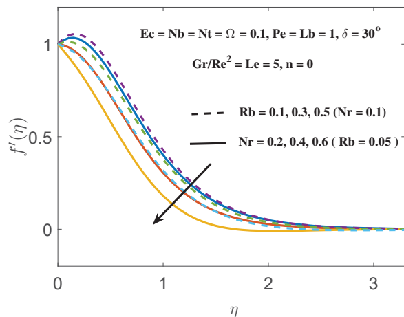
Fig. 4 Impact of Nr and Rb on f'(\eta)
