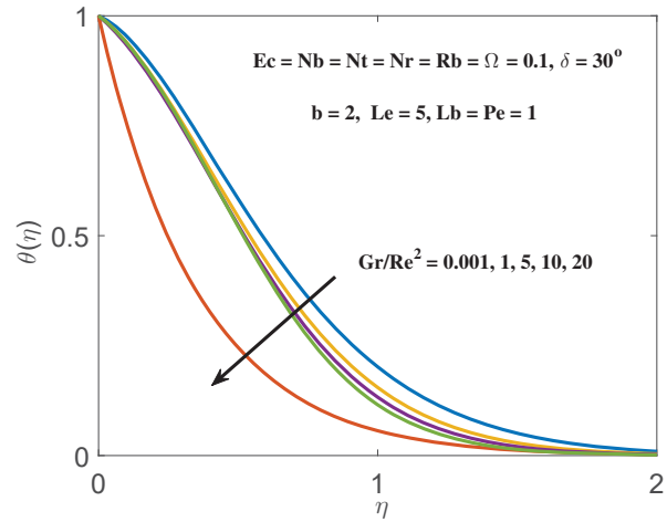
Fig. 6 Impact of \frac{Gr}{Re^2} on \theta(\eta)
