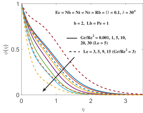
Fig. 10 Impact of \frac{Gr}{Re^2} and Le on \phi(\eta)
