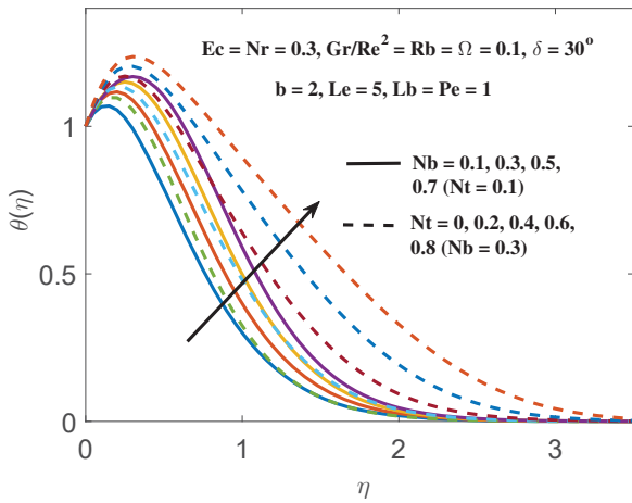
Fig. 8 Impact of Nb and Nt on \theta(\eta)
