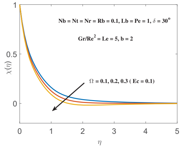
Fig. 16 Effect of \Omega on \chi(\eta)
