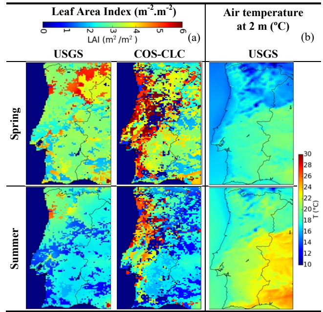
Fig. 4 (a) Average Leaf Area Index ( m^2 \cdot m^{-2} ) for the spring and summer using both LC approaches; (b) 2 m average air temperature ( ^{\circ}C ) for the spring and summer using the USGS LC approach
