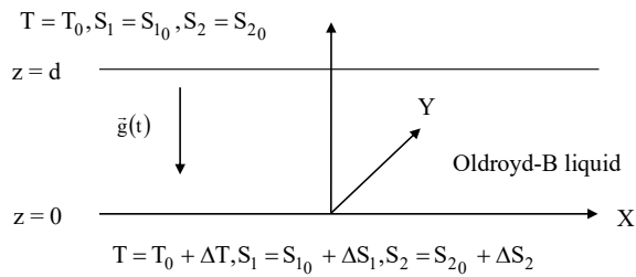
Fig. 1 Physical configuration of triple diffusive convection in Oldroyd-B liquid under gravity modulation where
