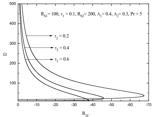
Fig. 7 Plot of R_{2C} versus \Omega for different values of ratio of diffusivity of solute2 and heat diffusivity \tau_2
