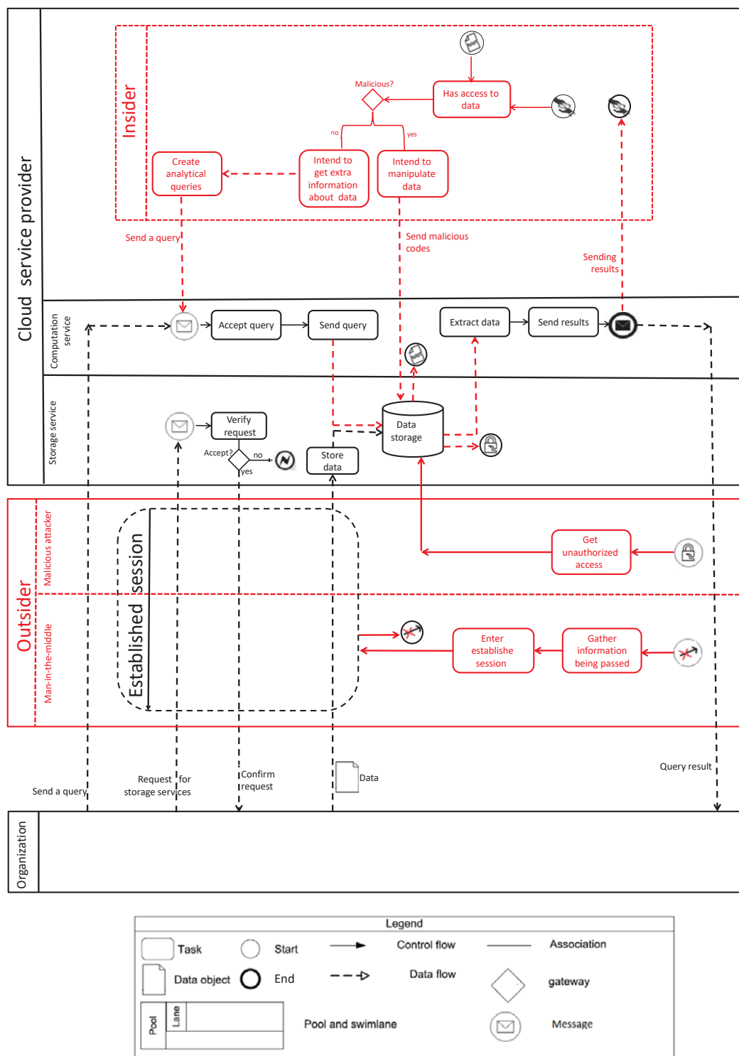
Fig. 2 Security threats in the cloud business processes
