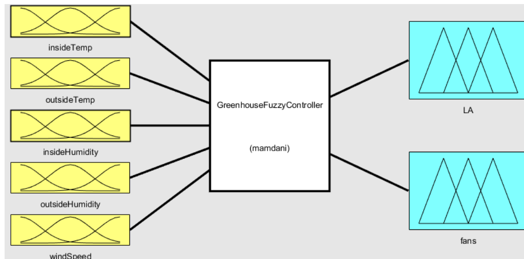
Fig. 2 Mamdani Fuzzy Controller Structure
