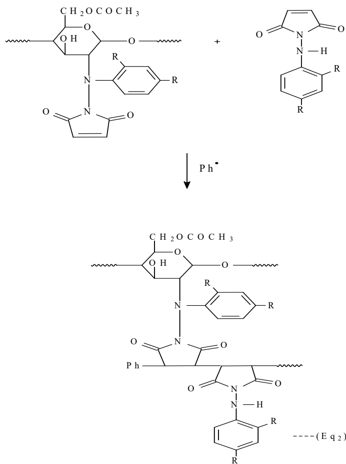
Fig. 3 Suggested reaction mechanism of the grafting process of APHM derivatives onto cellulose acetate
