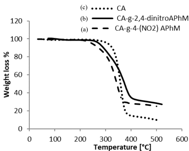
Fig. 8 Thermogravimetry (TG) of CA grafted with (a) 4-(NO 2 )APhM 6.66 % and (b) 2,4-di (NO 2 ) APhM 20 % as compared that of CA (c)
