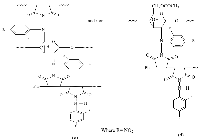
Fig. 4 Suggested reaction mechanism of the grafting process of 2,4-di (NO 2 )PhAM onto cellulose acetate
