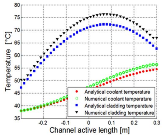
Fig. 6 The coolant and cladding temperatures variations along the hot channel
