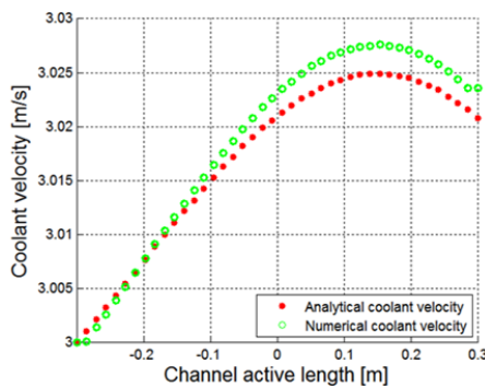
Fig. 1 A comparison between the analytical steady state and transient numerical coolant velocity
