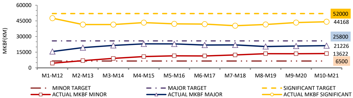
Fig. 3 Reliability demonstration based on actual fleet distance achieved
