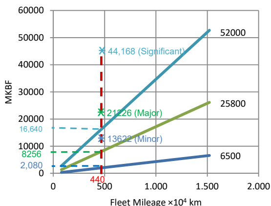
Fig. 5 Yearly Distance accumulated versus MDBF target
