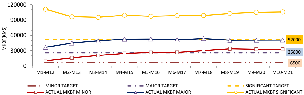
Fig. 4 Reliability demonstration based on design operational profile
