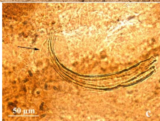
Fig. 2 Filaroides martis found in the lungs from a stone marten from Bulgaria: a) Anterior end. b) Spicules (under compression) – proximal end (1), distal end (2). c) Spicules and gubernaculum (the arrow) under compression
