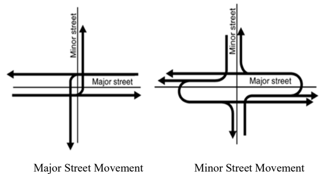
Fig. 2 Superstreet Traffic Movement [3]
