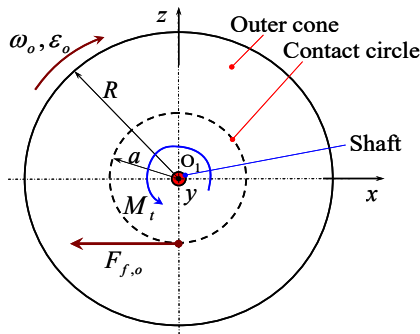
Fig. 4 Equilibrium of moments on the outer cone around O_1y axis
