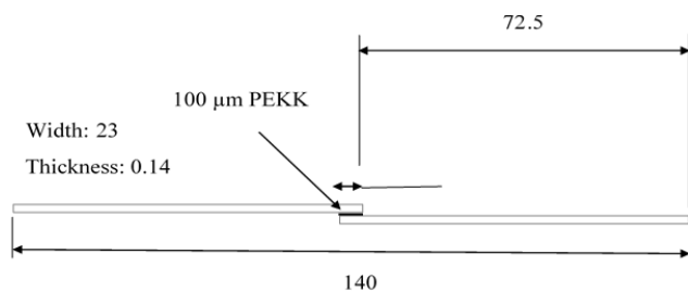
Fig. 1 Lab shear specimens (dimensions in mm)
