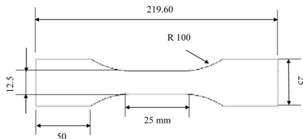
Fig. 4 Specimen geometry (dimensions in mm) [9]
