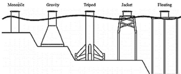
Fig. 1 Offshore wind turbines foundations [8]
