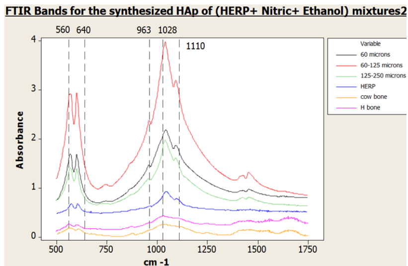
Fig. 5 FTIR spectra of the synthesized HAp materials of (HERP + dil.Nitric + Ethanol) mixtures, 500 \text{cm}^{-1} to 1750 \text{cm}^{-1}
