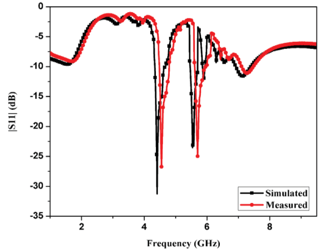
Fig. 6 Reflection coefficient |S_{11}| versus frequency, when D1 is “OFF” and D2 is “ON”
