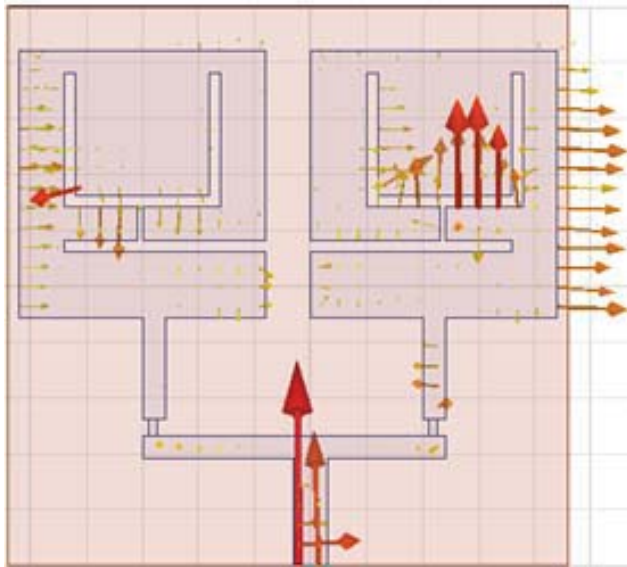
Fig. 8 Current distribution of proposed antenna array
