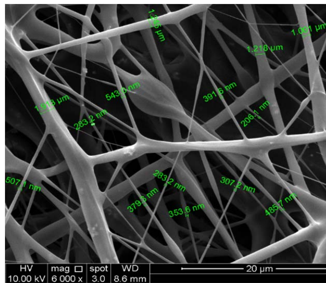
Fig. 1 (c) SEM of \text{Bi}_2\text{O}_3/\text{epoxy-PVA} nanofibers, using 0.21 mm ID of needle
