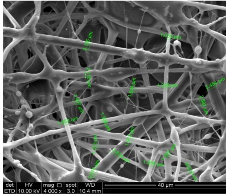
Fig. 1 (b) SEM of \text{Bi}_2\text{O}_3/\text{epoxy-PVA} nanofibers, using 0.26 mm ID of needle
