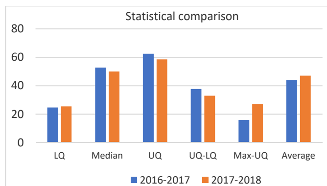
Fig. 3 Statistical Comparison
