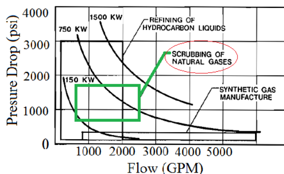
Fig. 14 Scope of the PRT technology
