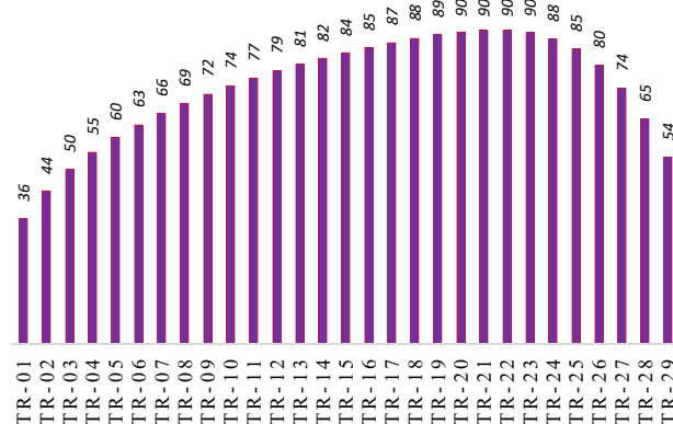
Fig. 3 Temperature profile of absorber column (°C)
