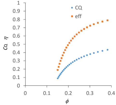
Fig. 12 Performance prediction of Wells turbine N_b = 4 , r_o / c = 5 , r_i / c = 1 , \sigma \approx 0.2 m_0 = 0.7 (C_i \equiv m_0 \times 2\pi \sin \alpha) , C_d = 0.1
