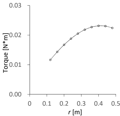
Fig. 11 Wells turbine radial torque distribution N_b = 4 , r_o = 0.5\text{m} , r_i = 0.1\text{m} , c=0.1\text{m} , V=3\text{m} , N=200\text{rpm} \sigma \approx 0.2 , m_0 = 0.7 (C_i \equiv m_0 \times 2\pi \sin \alpha) , C_d = 0.1
