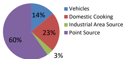
Fig. 3 Emission Inventory for PM_{2.5}
