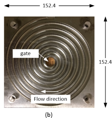
Fig. 2 (a) Injection system and (b) spiral mold (dimensions in millimeters)
