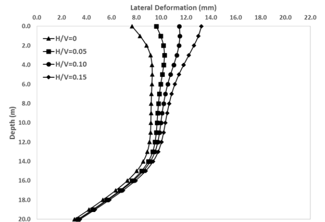
Fig. 9 Effects of inclined loading on rear pile row lateral deformation
