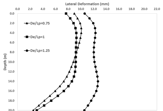
Fig. 5 Effects of final excavation depth on rear pile row lateral deformation
