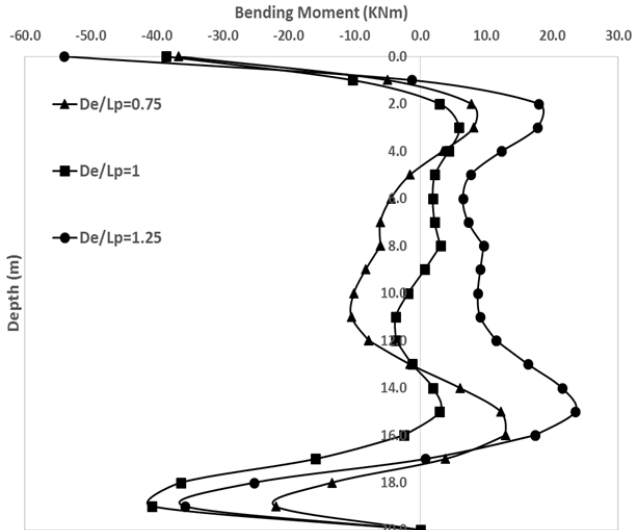
Fig. 6 Effects of final excavation depth on front pile row bending moment
