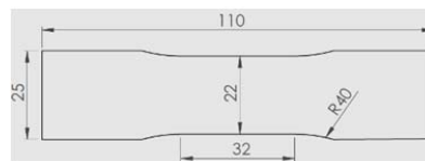
Fig. 2 Specimen geometry for tests using anti-buckling fixture
