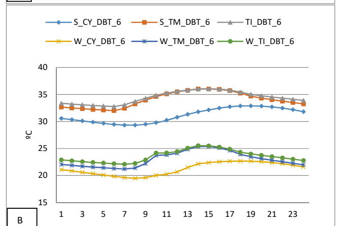
Fig. 4 IAT of various building fabrication of zones 1 (A), 6 (B) in both summer and winter
