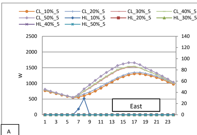
Fig. 2 Heating and Cooling Loads of various glazing to wall ratio in zones 1 (A), and 2 (B)
