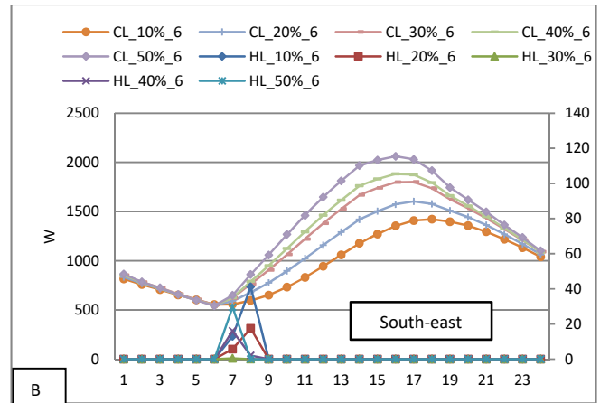
Fig. 3 Heating and Cooling Loads of various glazing to wall ratio in zones 5 (A), and 6 (B)
