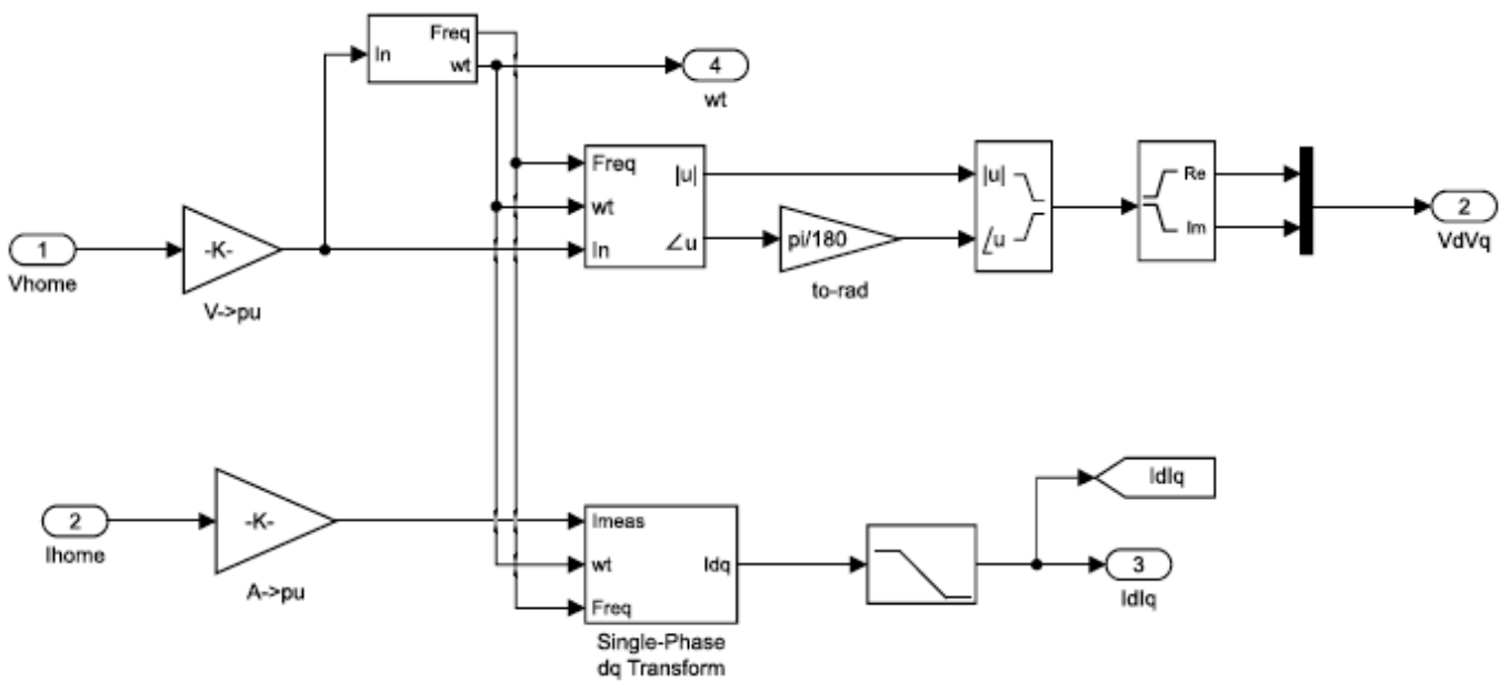
Fig. 5 PLL measurements
