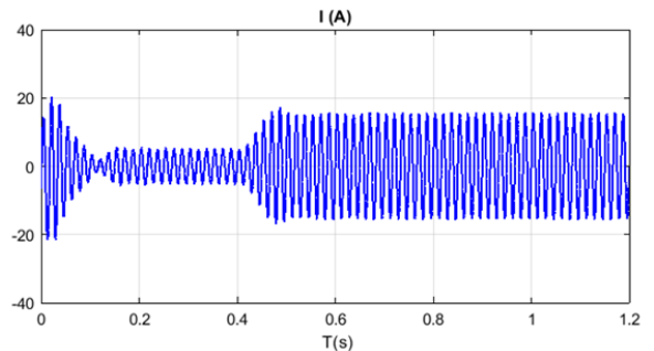
Fig. 13 Grid current
