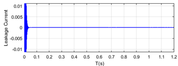
Fig. 18 Leakage current at Rg
