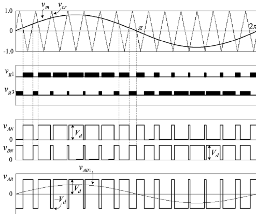
Fig. 3 Bi-polar PWM waveforms
