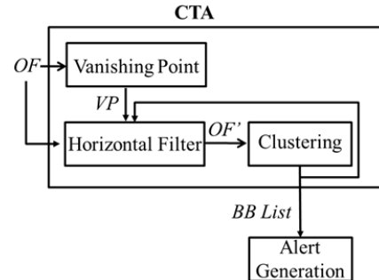
Fig. 2 Block based schema of the CTA algorithm
