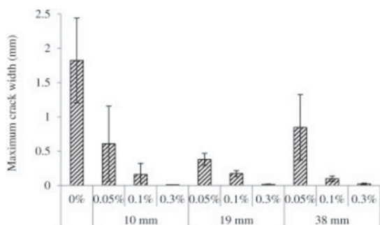
Fig. 2 L Flax Fiber Length and Volume [20]
