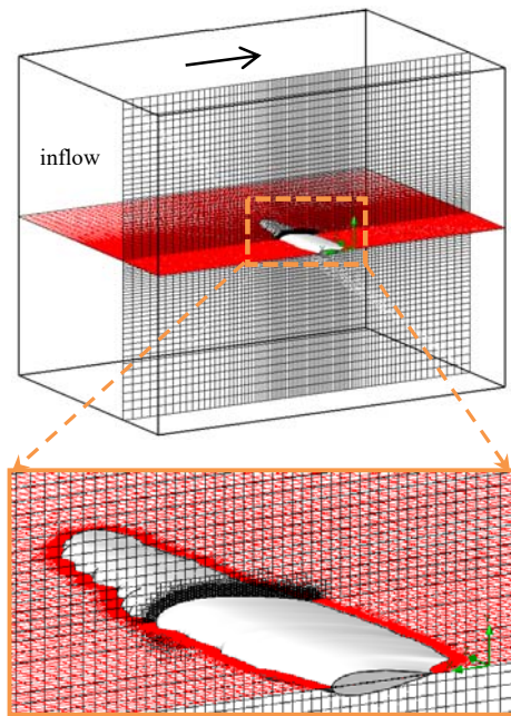
Fig. 18 Humpback whale flipper grid and computational domain
