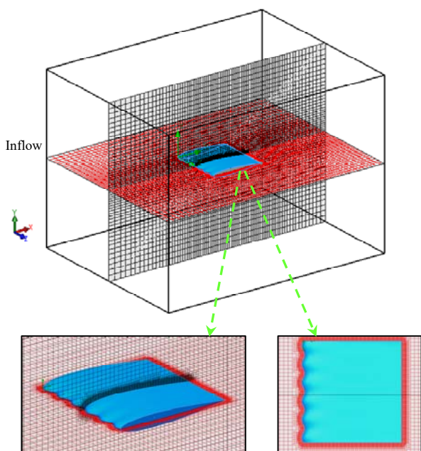
Fig. 11 Tubercled wing grid and computational domain
