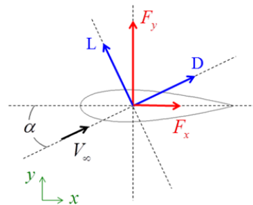
Fig. 10 Airfoil section coordinate system
