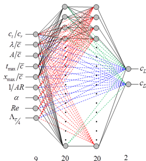
Fig. 4 Topology of the designed cascade-forward ANN
