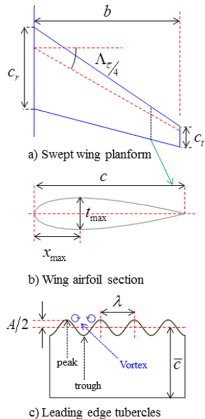
Fig. 3 Wing planform anatomy and its characterizing parameters
