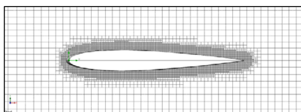
Fig. 12 Cross-sectional adaptive grid around NACA 0012 airfoil
