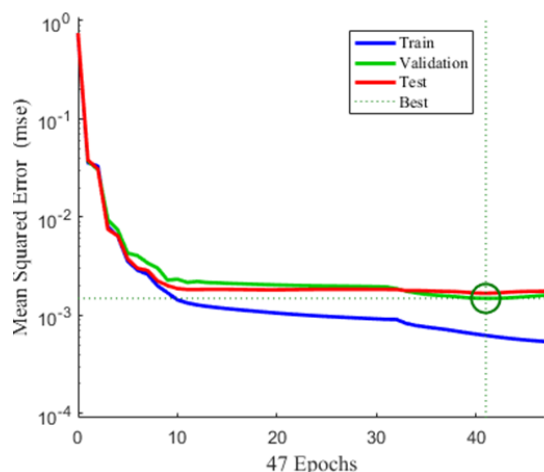
Fig. 5 Learning history of the designed cascade-forward ANN
