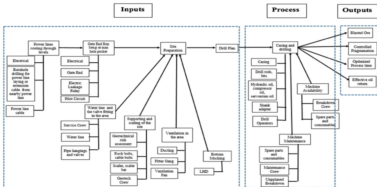
Fig. 3 Process map of production drilling operation
