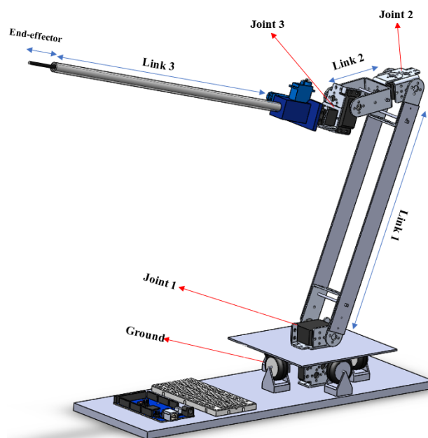
Fig. 1 Robot-assisted laparoscope and its links and joints
