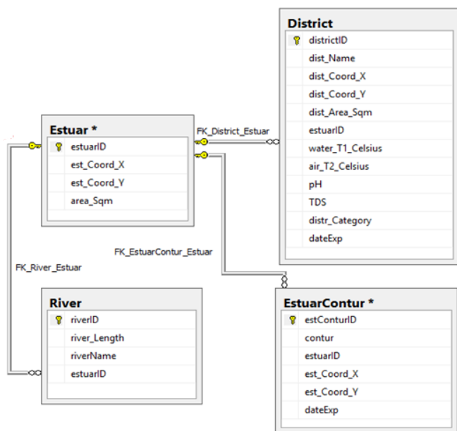
Fig. 4 ERM- Conceptual Model
