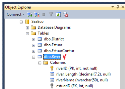
Fig. 5 The tables in SQL Server
