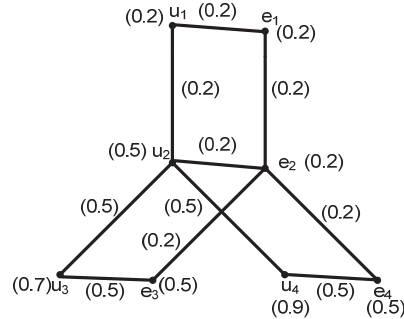
Fig. 11 Double Layered Non-Cyclic Fuzzy Graph NCDL (G) = (\sigma_{NCDL}, \mu_{NCDL})
