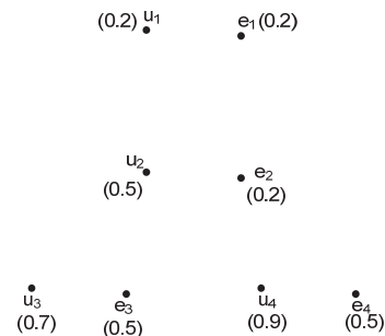
Fig. 12 Complement of Double Layered Non-Cyclic Fuzzy Graph NCDL(G^\mu) = (\sigma^\mu_{NCDL}, \mu^\mu_{NCDL})
