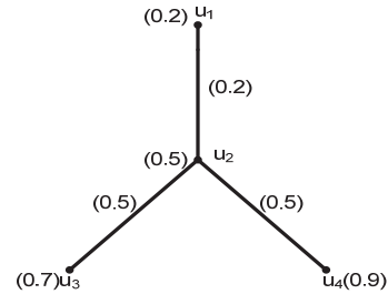
Fig. 10 Fuzzy Graph G : (\sigma, \mu) whose crisp graph G^* : (\sigma^*, \mu^*) is a non-cycle
