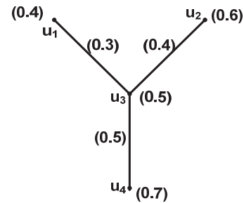
Fig. 3 Fuzzy Graph G : (\sigma, \mu) whose crisp graph G^* : (\sigma^*, \mu^*) is a non-cycle
