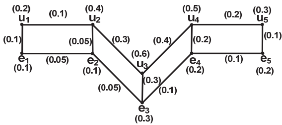
Fig. 6 Double Layered Non-Cyclic Fuzzy Graph NCDL (G) = (\sigma_{NCDL}, \mu_{NCDL})
