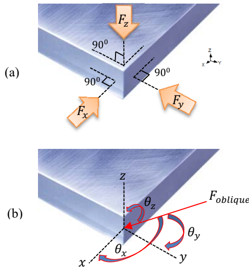
Fig. 1 (a) Normal impact ( F_x, F_{1y}, & F_{1z} ) and (b) oblique impact ( F_{oblique} ) acting on a plate
