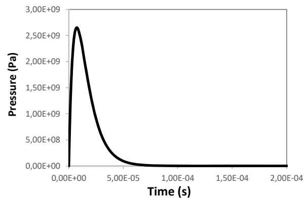
Fig. 2 Explosion pressure pulse
