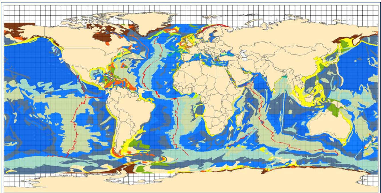
Fig. 8 The global seabed sediment maps 10 th edition Shom Ed., 2017
