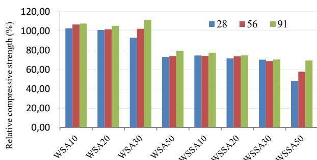
Fig. 6 Relative compressive strength of mortars with biomass ashes at the different ages
