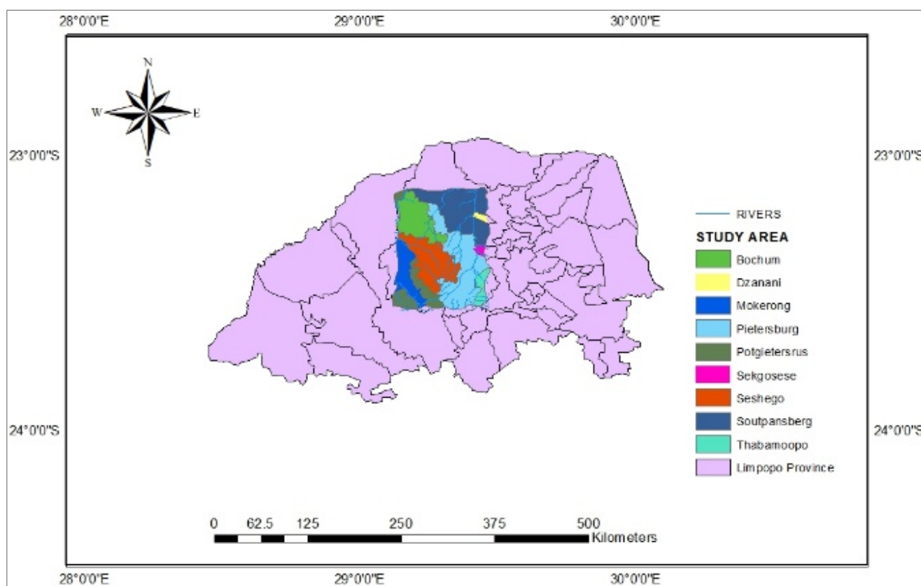
Fig. 1 Study area location map
