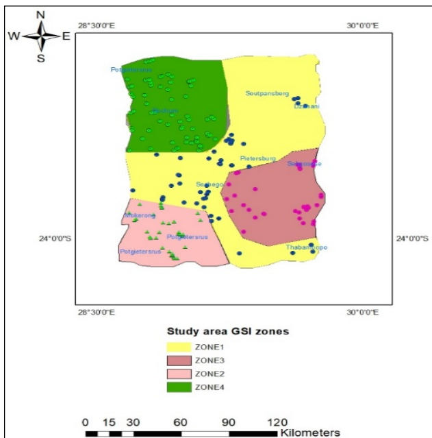
Fig. 3 Demarcation of GSI zones
