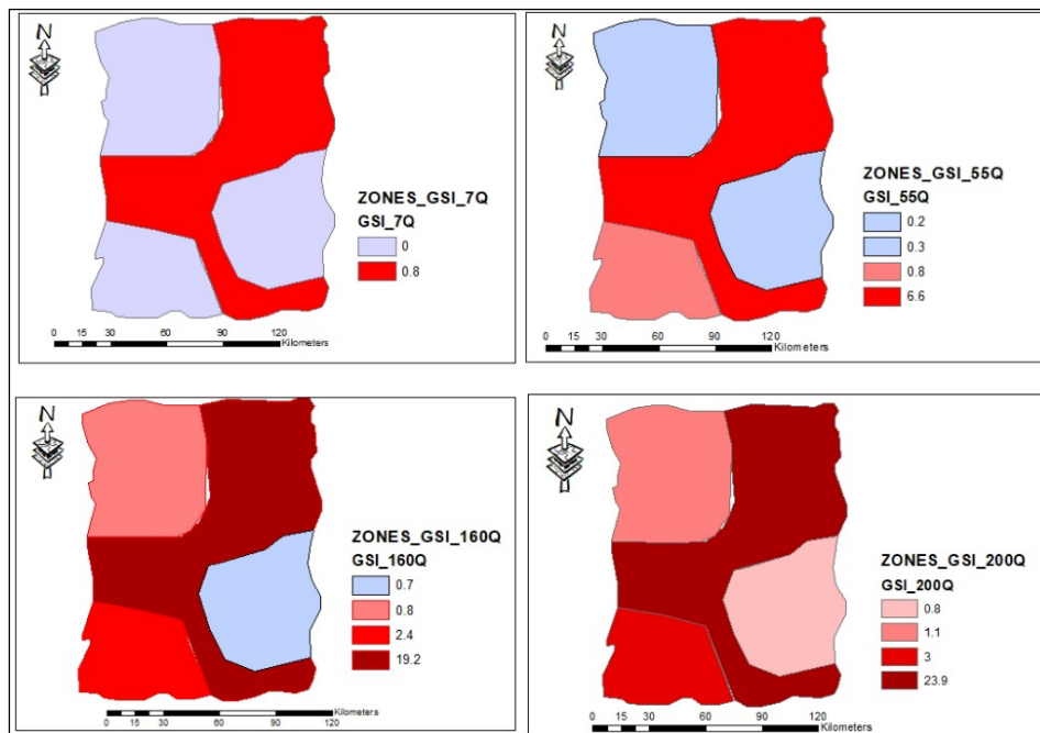
Fig. 6 GSI analysis for four zones
