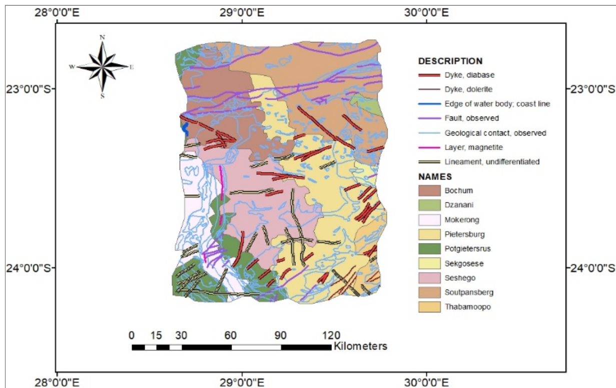
Fig. 2 Geological structures map.
