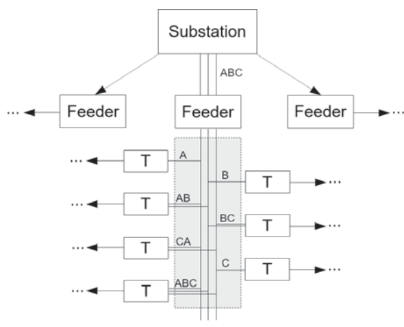
Fig. 1 Hierarchical levels of a power distribution circuit
