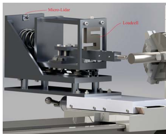
Fig. 1 Schematic of the circular shaft Tribometer
