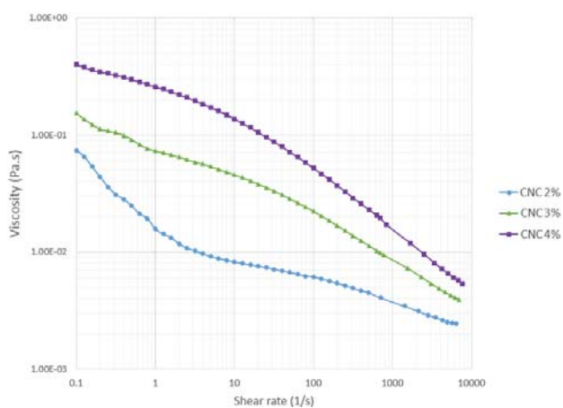
Fig. 8 viscosity profile of CNC suspensions versus shear rate
