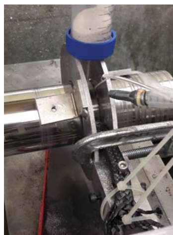
Fig. 2 Experimental setup with packing material and sands
