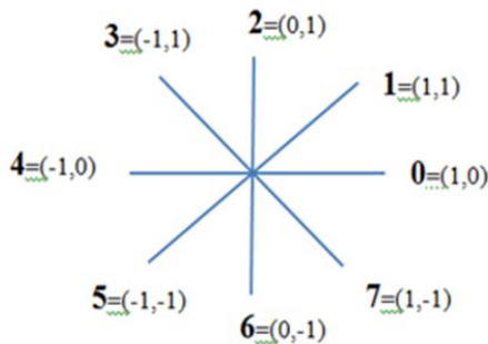
Fig. 6 Eight-direction chain code
